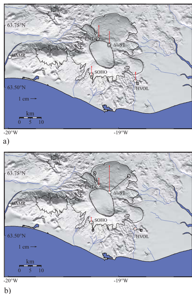
Figure 15. Predicted displacements induced by ice unloading around Katla from 2001 June to 2004 June. Uplift (red arrows) and horizontal displacement (black arrows) are shown at AUST, ENTA, SOHO and HVOL relative to HAMR. (a) Model of ice unloading (parameters used are the same as in Fig. 14). (b) Difference between displacements observed (see Fig. 6) and the ice unloading model. Outline of icecaps are shown.
